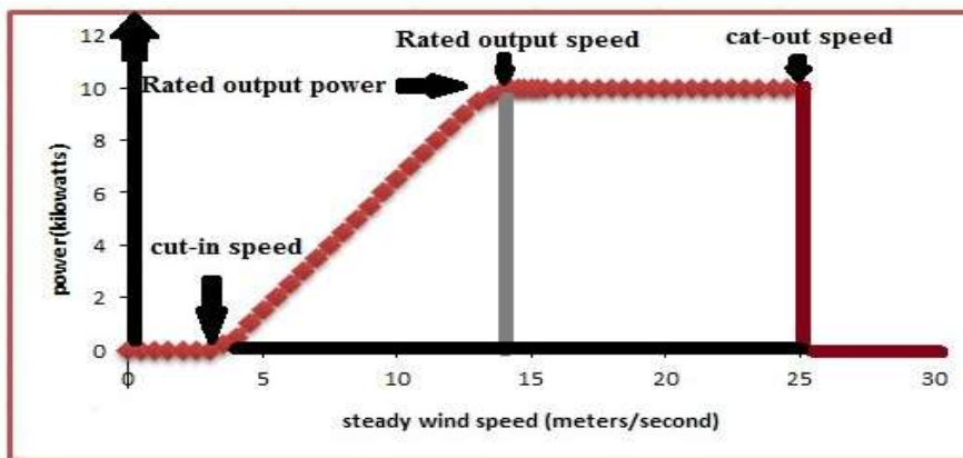
Fig. 1. wind speed with power output [14].
