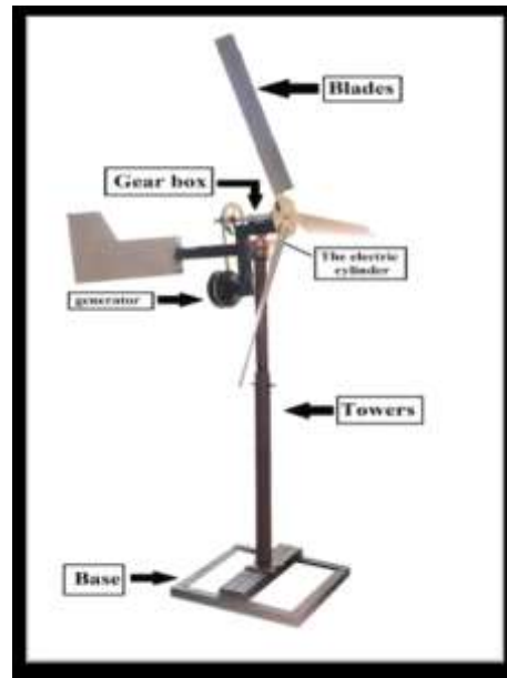
Fig. 3. Assembly wind turbine component.
