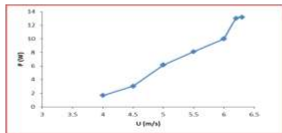
Fig. 7. Relation between wind speed and power.
