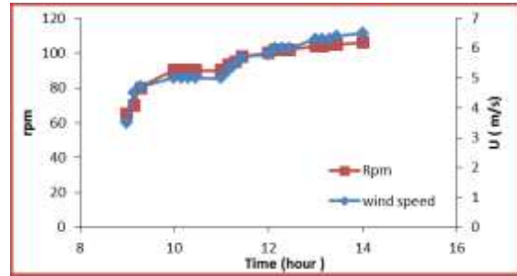
Fig. 6. Relation between time with wind speed and rpm.
