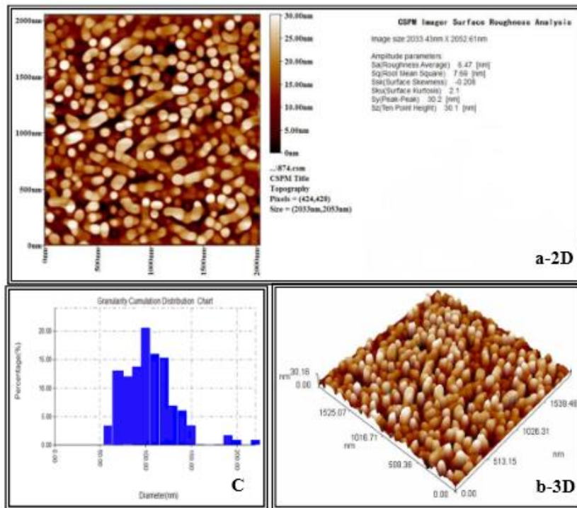
Fig. 5: Measure of (AFM) for sample of alloy (A)
