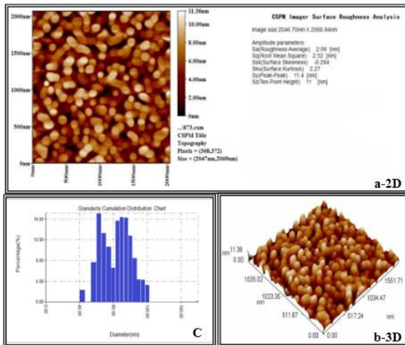
Fig. 6: Measure of (AFM) for sample of alloy (B)
