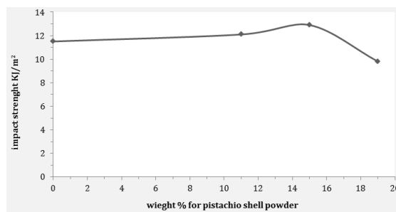
Fig.6: Impact strength and absorbed energy versus Pistachio shell content
