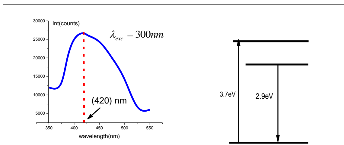
Fig.(5-c): The energy levels and photoluminescence spectra for sample prepared (CaF 2 ) with (20 sec) for X-ray
