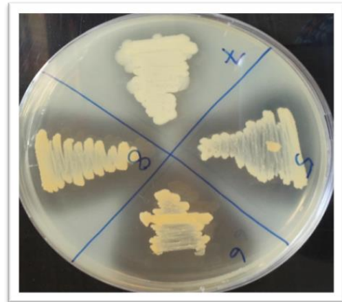
Fig.(4): The DNase production (clear zone around colonies)
