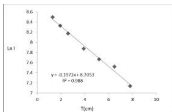
Fig. 7: Relationship between thickness T(cm) and Ln I for direct measurements of Cu at the 1173keV gate.
