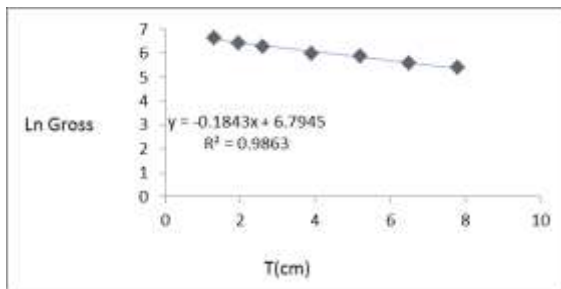
Fig. 9: Relationship between thickness T(cm) and Ln Gross for coincidence measurements of Cu at the 1173keV gate.
